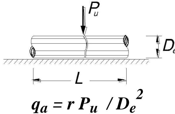
Figure 5. Point load testing. q_a = Allowable bearing pressure, kN / m 2 ; P_u = Crushing Point load acting laterally; D_e = Effective diameter of the soil 'rock' sample, D_e = (4A / \pi)^{0.5} ; A = Cross – sectional area of the irregular soil sample; r = Quality parameter, r = 2.4 for weathered and jointed soft rocks, r = 7.2 for reliable hard rock. An appropriate value is selected by engineering judgment for other samples and L \geq 1.5 D_e , ( L = Length of soil 'rock' sample).
