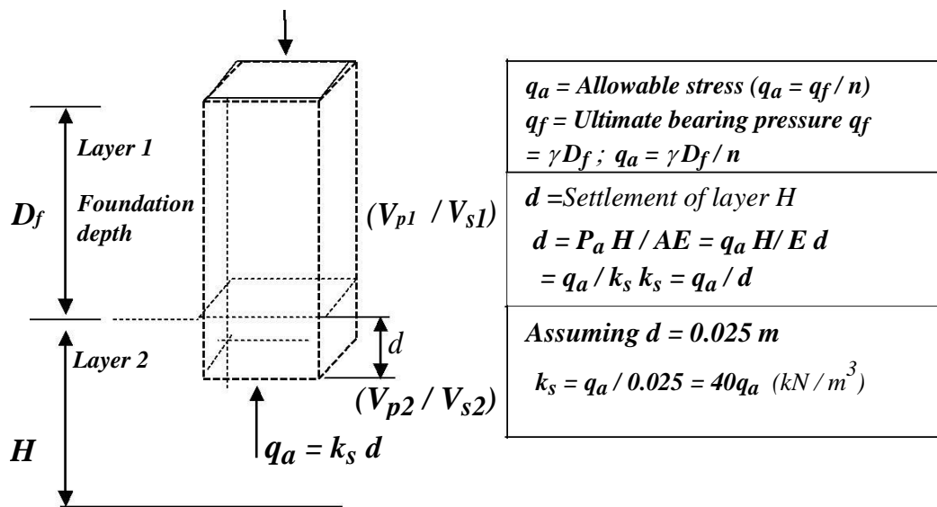
Figure 1. Soil column and related parameters.
