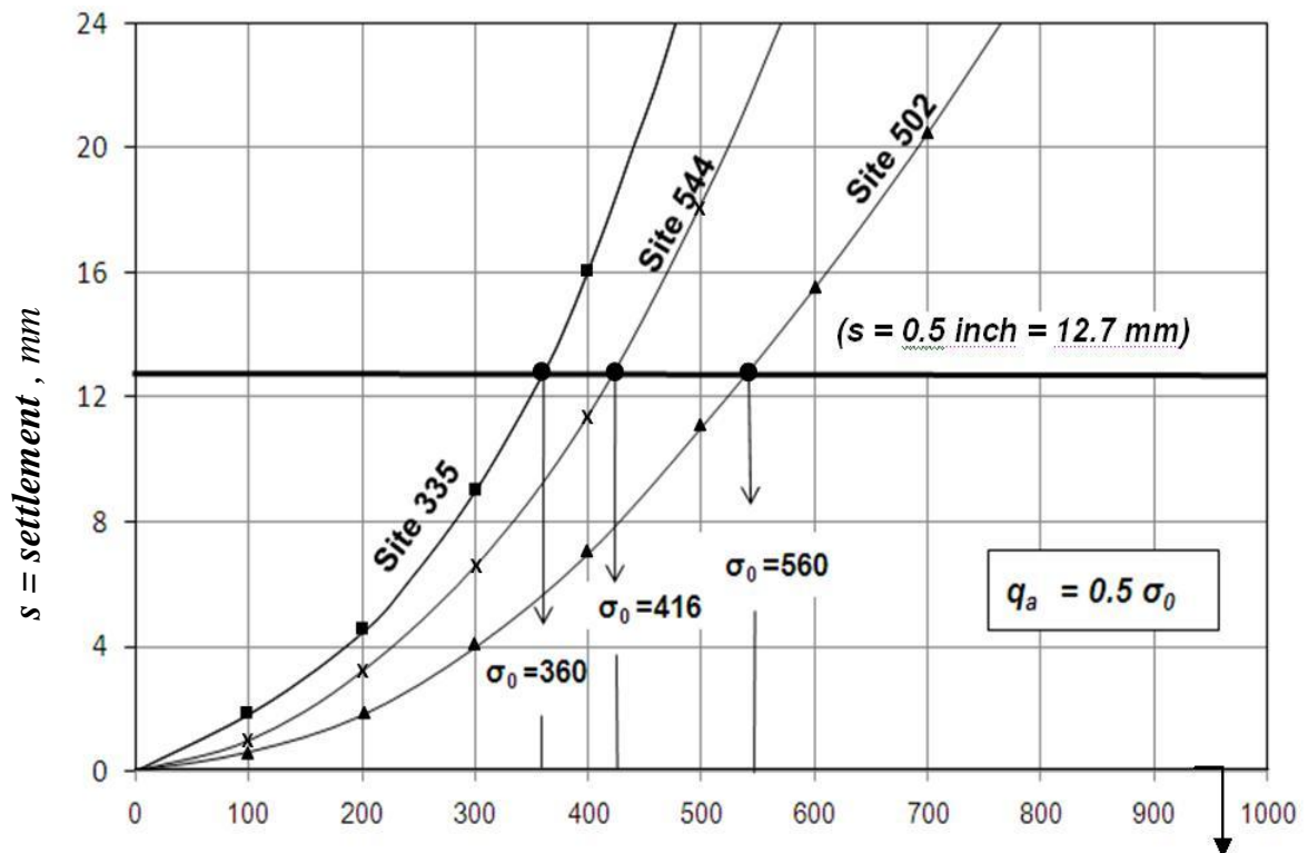
Figure 4. Load test results at Sites No: 335, 502, and 544. \sigma = \text{pressure under the test plate, kPa} ; ( \sigma_0 = 2 q_a = \text{pressure, which produces } s = 12.7 \text{ mm} ).
